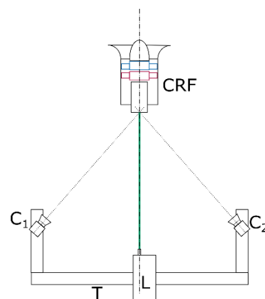
Figure 7: Experimental setup for outlet velocity measurement using particle image velocimetry (left) and schematic drawing (right)
